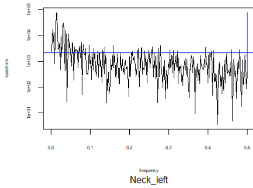
Fourier Spectrum Original OgaShin_06
