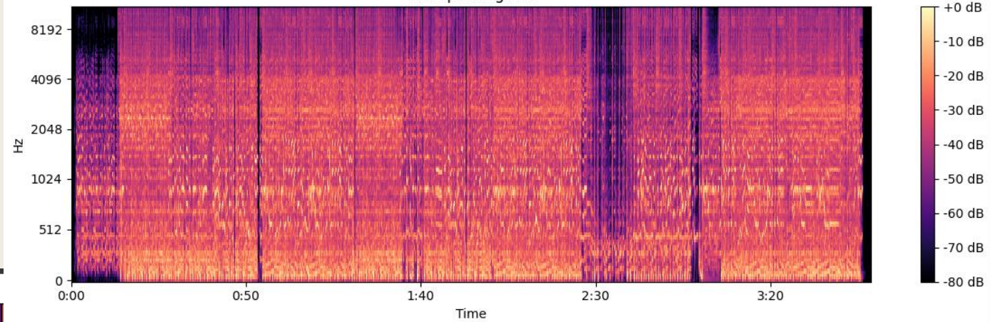
Mel spectrogram
