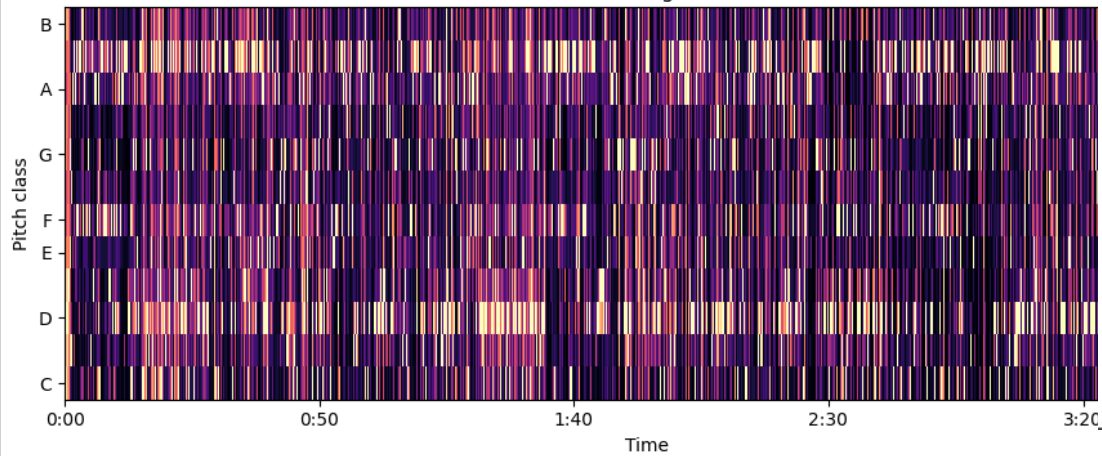
Chromagram
