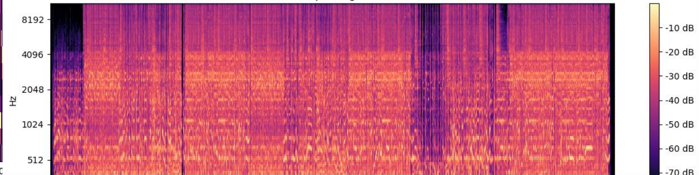
Mel spectrogram
